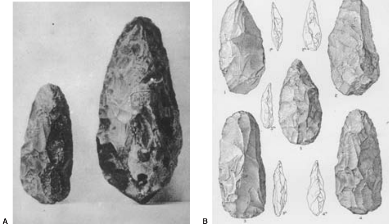
FIGURE 2.1 Left, G. F. Wright's (1890) composite image of the Newcomerstown paleolith alongside a paleolithic biface (reduced to one-half size) from Amiens, France; right, Holmes' (1893b) depiction of the Newcomerstown specimen alongside "four ordinary rejects." Holmes left it to the reader to decide which of the five specimens was from Newcomerstown, and which were quarry rejects. (From Wright 1890, Holmes 1893b.)
